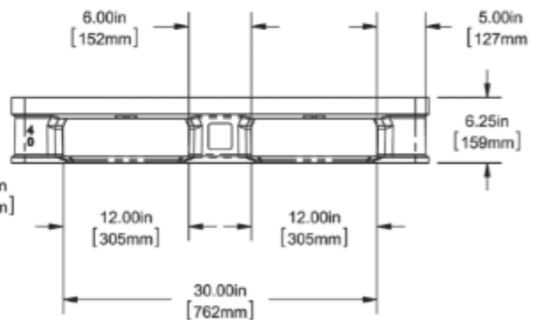
SIDE VIEW - 40"
