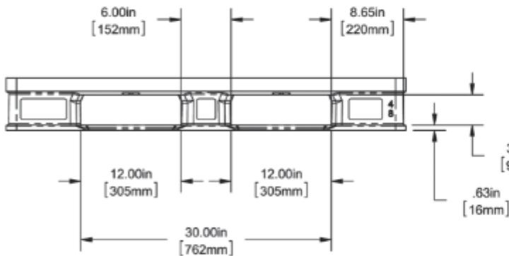
SIDE VIEW - 48"
